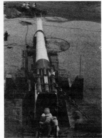
Scientists from McGill university push the first test slug into the breach, pith helmets were issued as part of the HARP uniform in what now looks like a comical colonial touch
